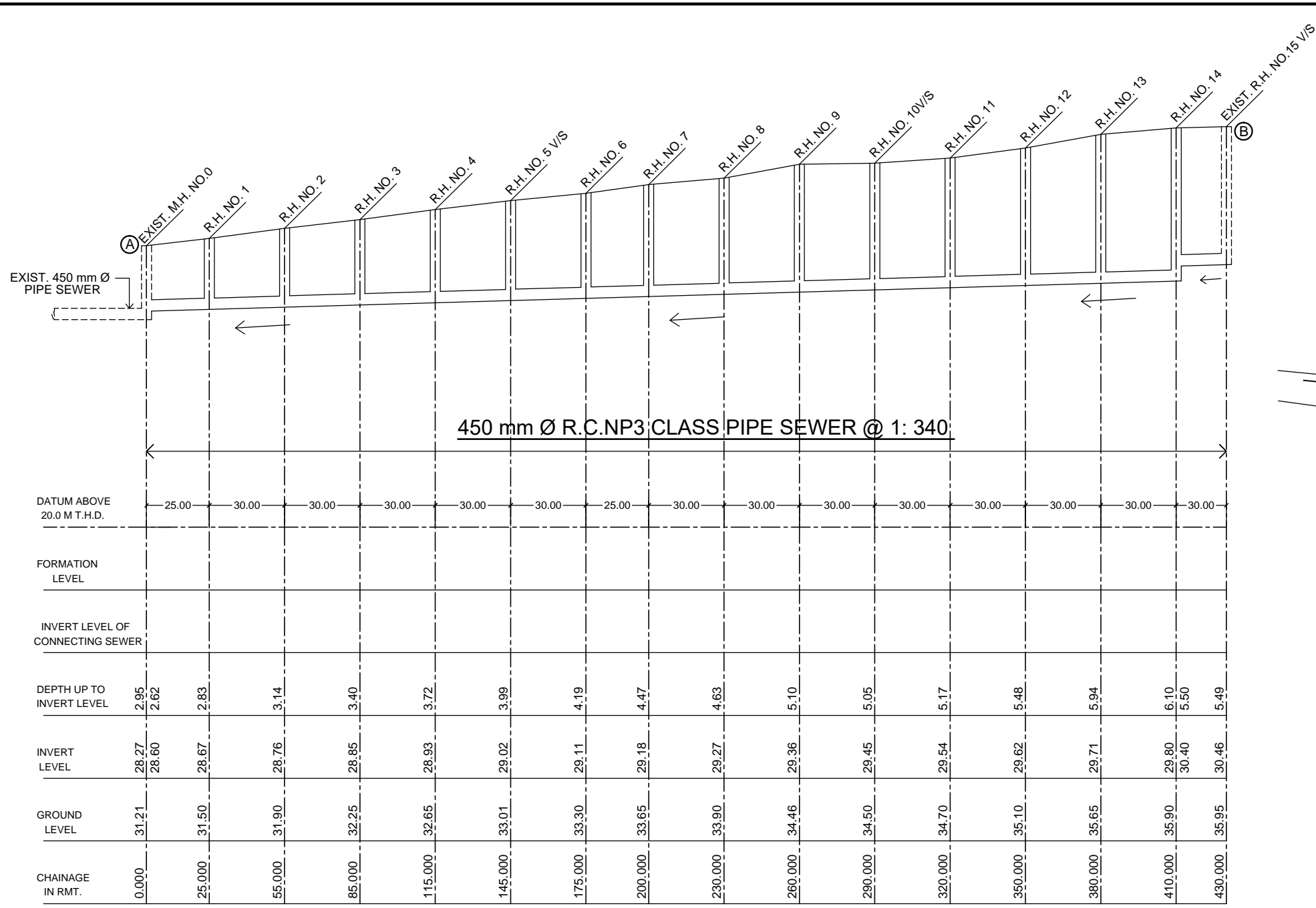
L - SECTION SCALE - VER.- 1cm = 1.0 mt HOR.- 1cm = 10.0 mt
